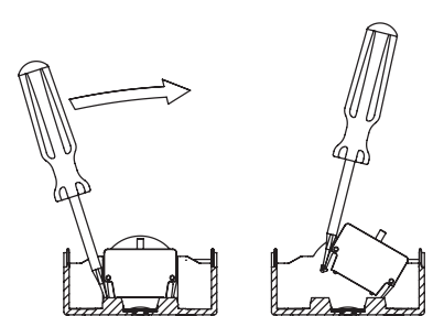
Contact block release from enclosure base
