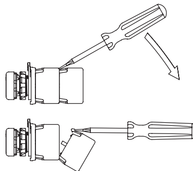
Contact block release from other block
