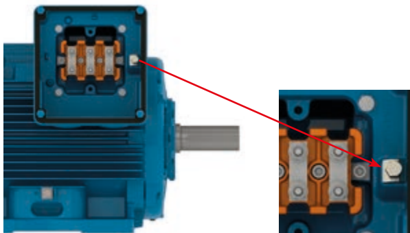
Figure 5 - Earth terminals in the terminal box
