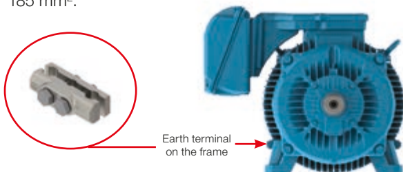
Figure 8 - Earth terminal position on the frame.
