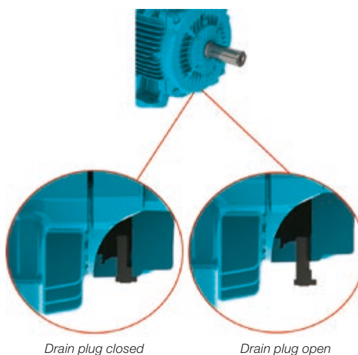
Figure 15 - Detail of the drain plug position on drive endshield
