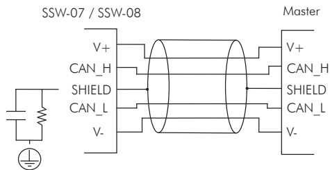
Figure 1 - DeviceNet connection
