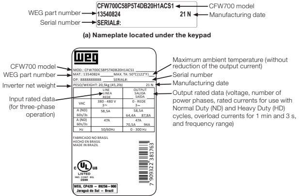
Figure 2: (a) to (b) - Identification label of the models CFW700...H1ACS1
