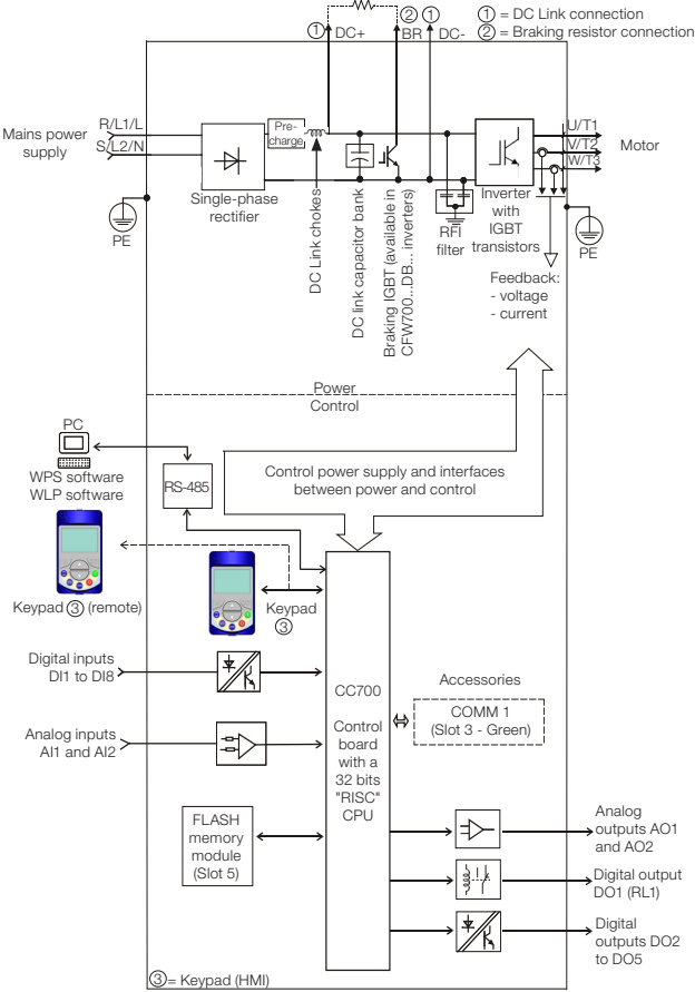
Figure 1: Block diagram of the CFW700...H1ACS1 models
