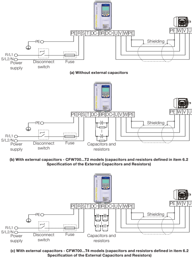
Figure 3: (a) to (c) - Power and grounding connections
