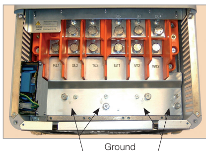
(e) Frame size E
