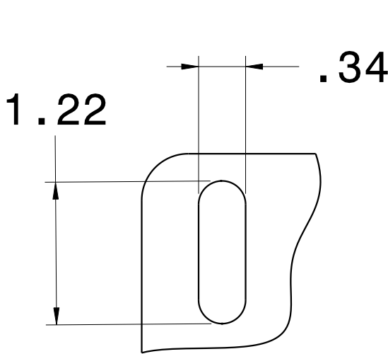
SLOT DETAIL 4X
