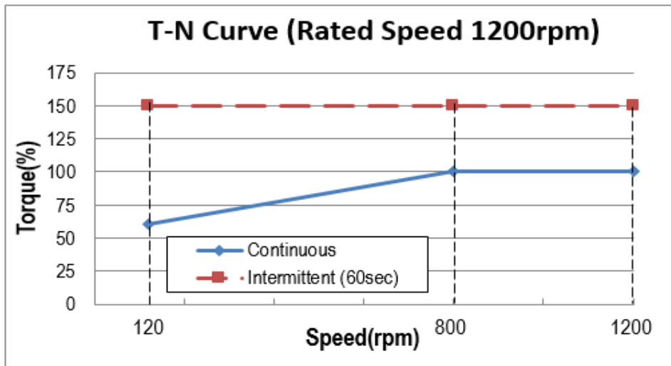
MOTOR T-N curve
