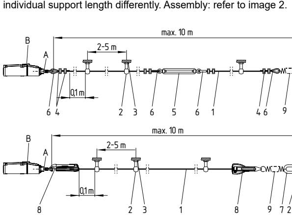
Image 2: Mounting of the components
