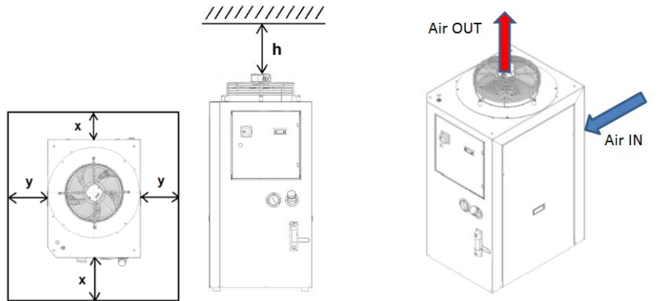
Picture 2 – Room minimum dimensions, x=h=1.5\text{ m} ; y=0.5\text{ m}
