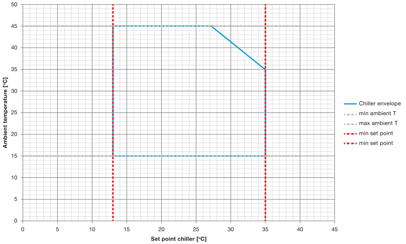
Operating limits - 50 Hz
