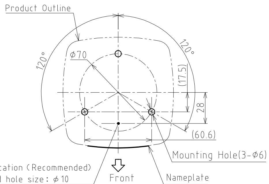
Installation Dimensions
