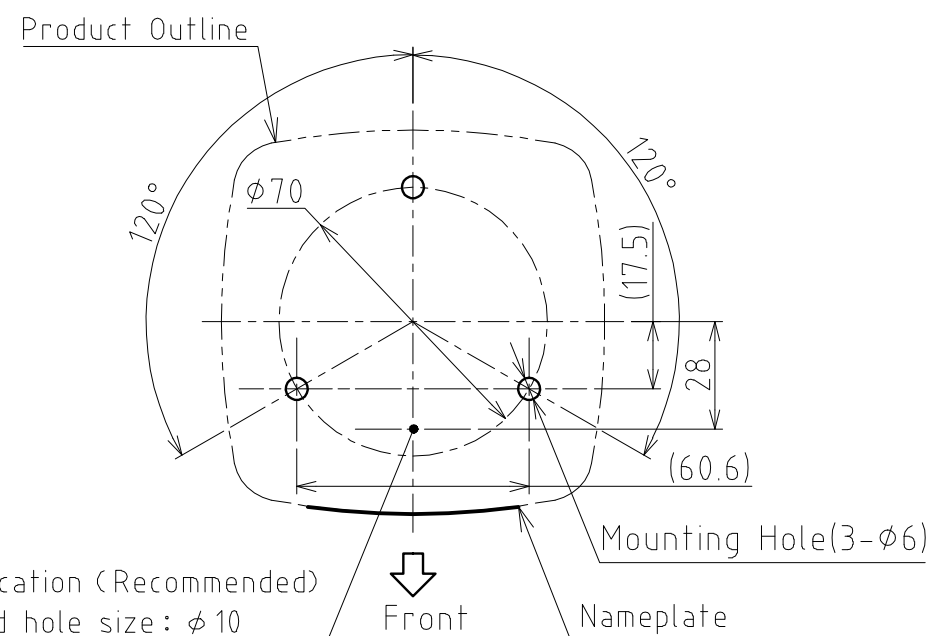
Installation Dimensions [1:2]
