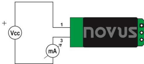
Fig. 4 – TxMini-M12 Connection Diagram
