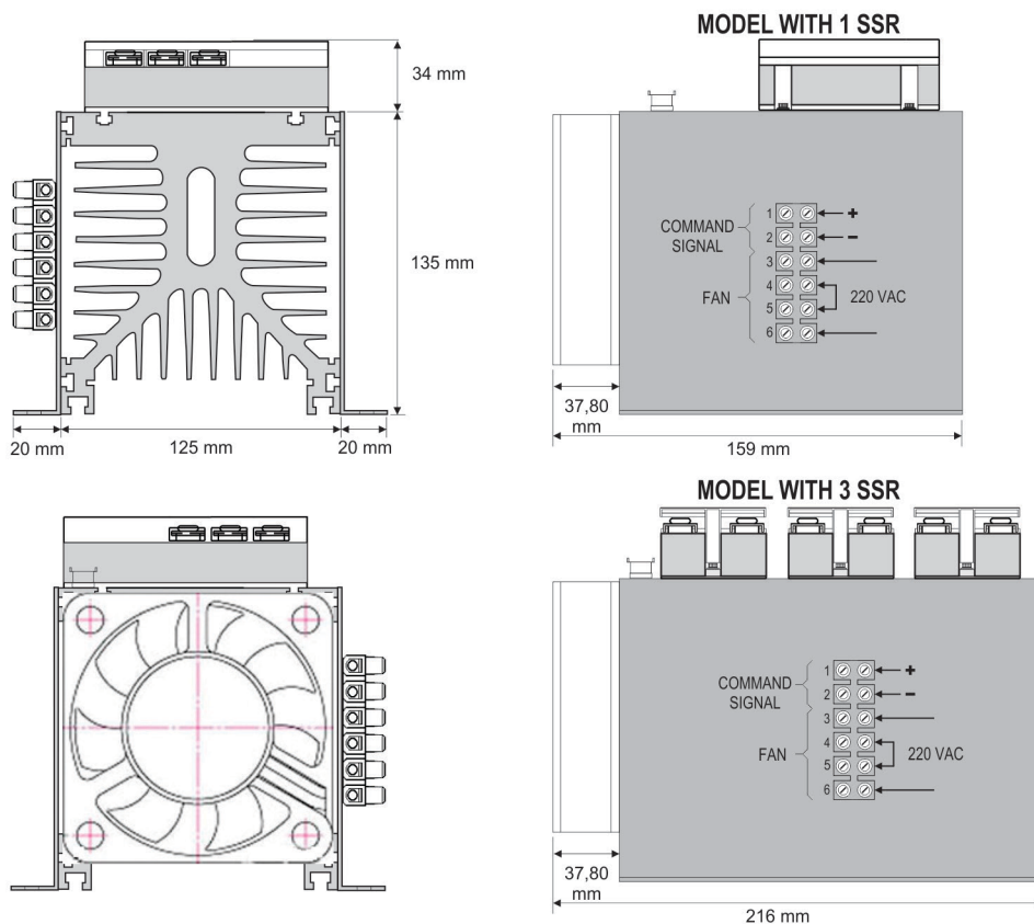
Fig. 07 – Dimensions of SSR static switch
