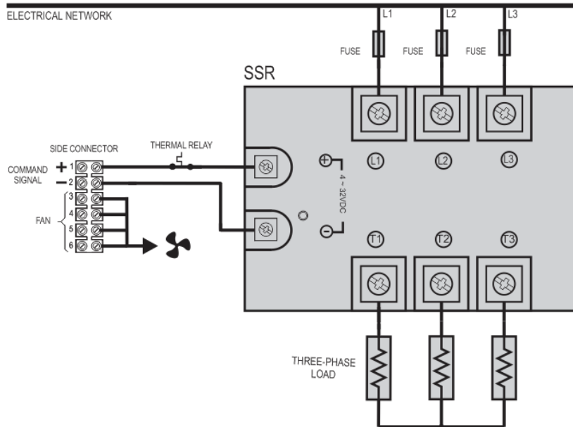
Fig. 05 – Electrical Connections - Command Signal and SSR Static Key Charge (1 SSR – 3F)
