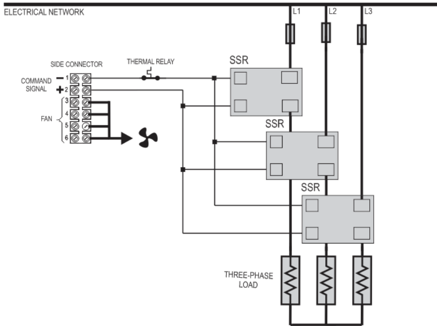
Fig. 04 – Electrical Connections - Command Signal and SSR Static Key Charge (3 SSR)
