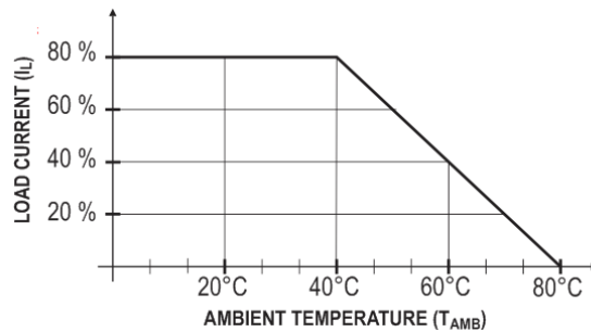
Fig. 06 – Ambient Temperature and Load Current
