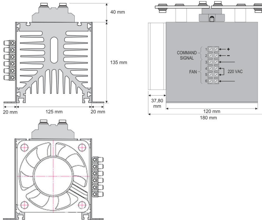
Fig. 06 – Heatsink NDP3 dimensions
