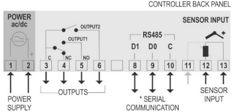
Fig. 1 - N322T terminals
