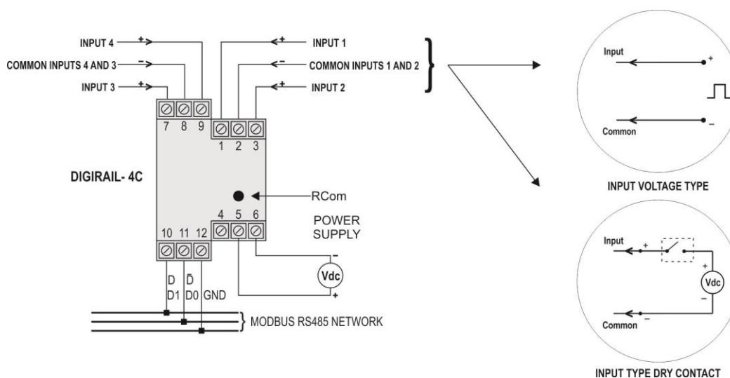
Figure 2 – Electrical Connections
