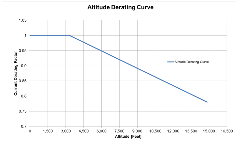
Figure 5-3: Altitude Derating Curve
