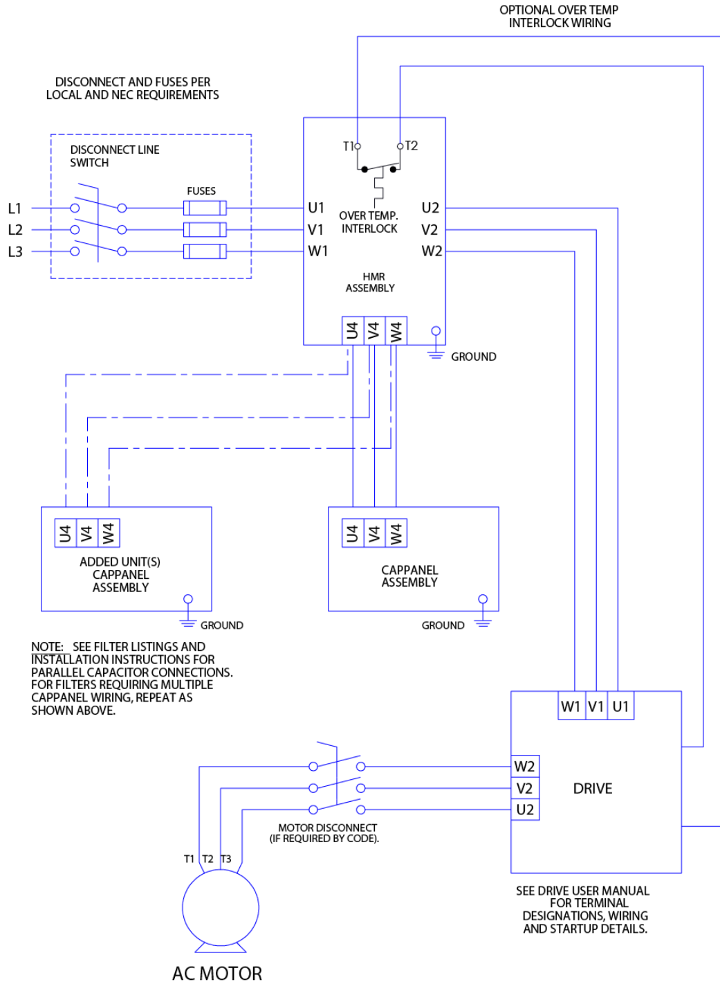
Figure 6-2: Open Panel Interconnection
