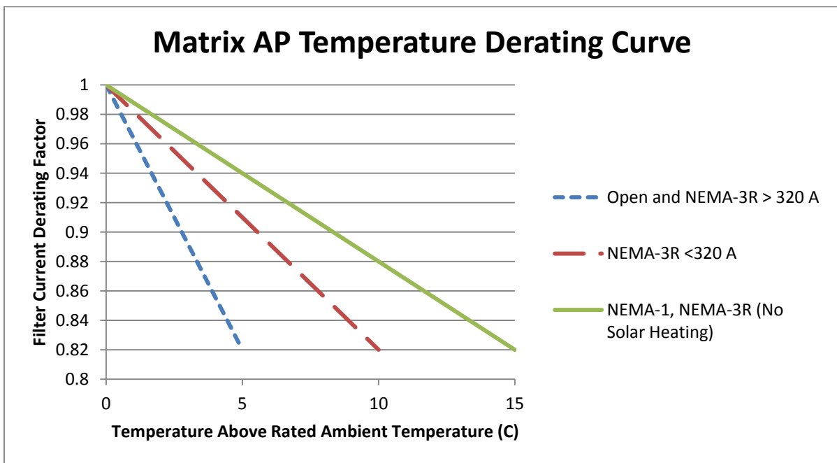
Figure 5-4: Temperature Derating
