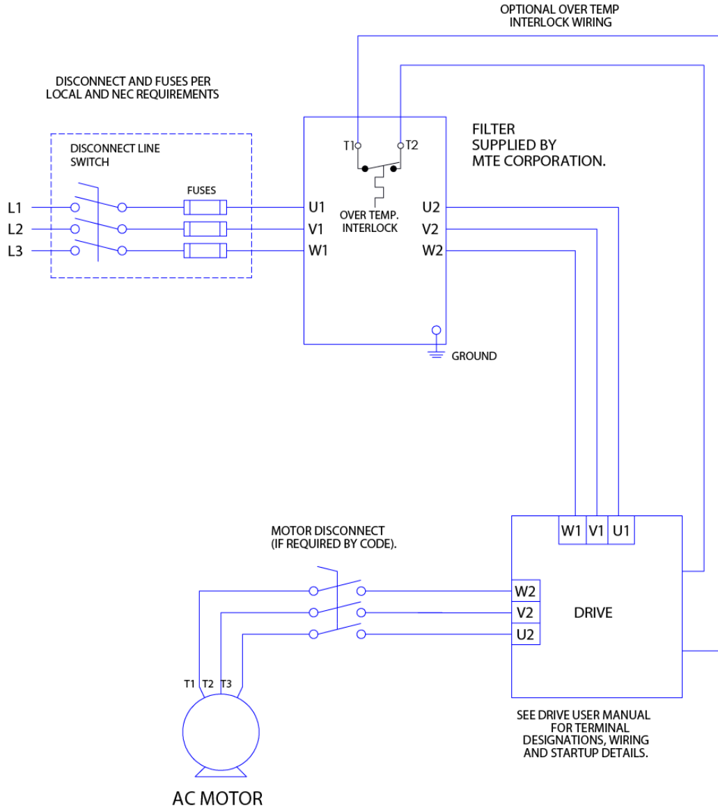
Figure 6-3: Enclosed Interconnection
