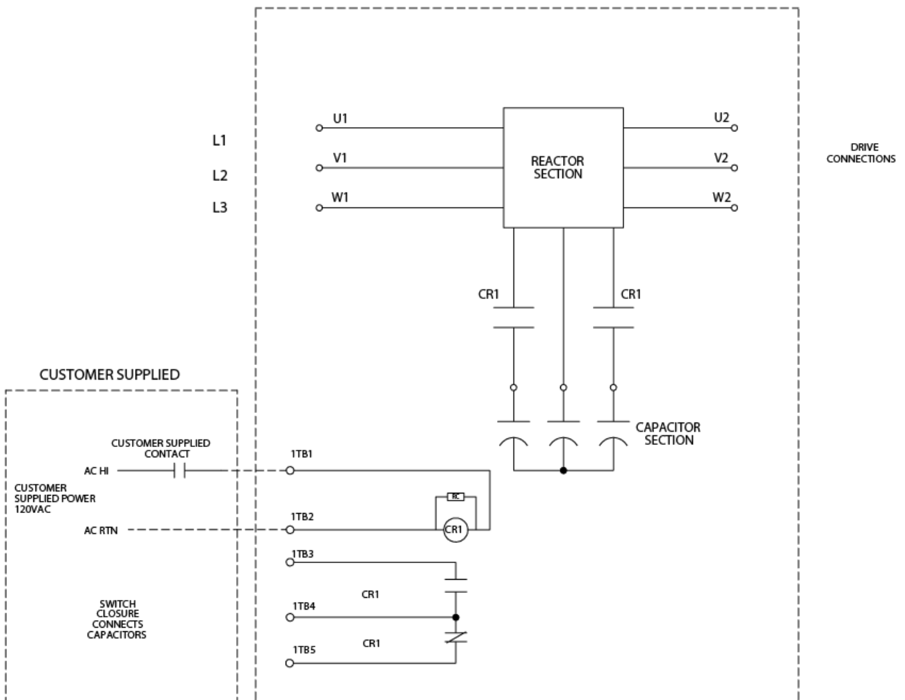
Figure 6-4: Contactor Options – 002
