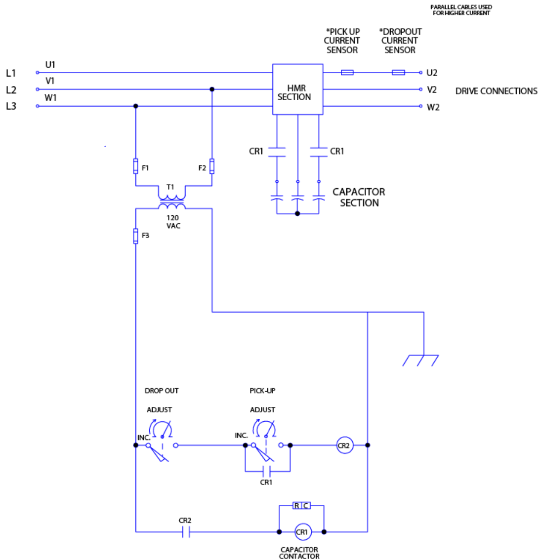
Figure 6-5: Contactor Option – 009
