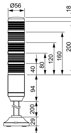
Buzzer Kit (MPZ-56E)
