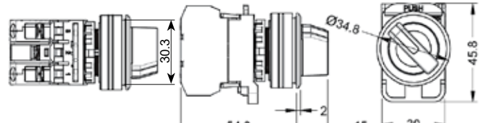
2/3 Position selector w/flush mountable metal bezels
