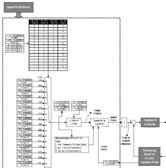
Figure 5-2 Speed profile block
