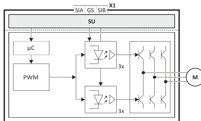
Fig. 11: Functional principle: Basic Safety - STO
