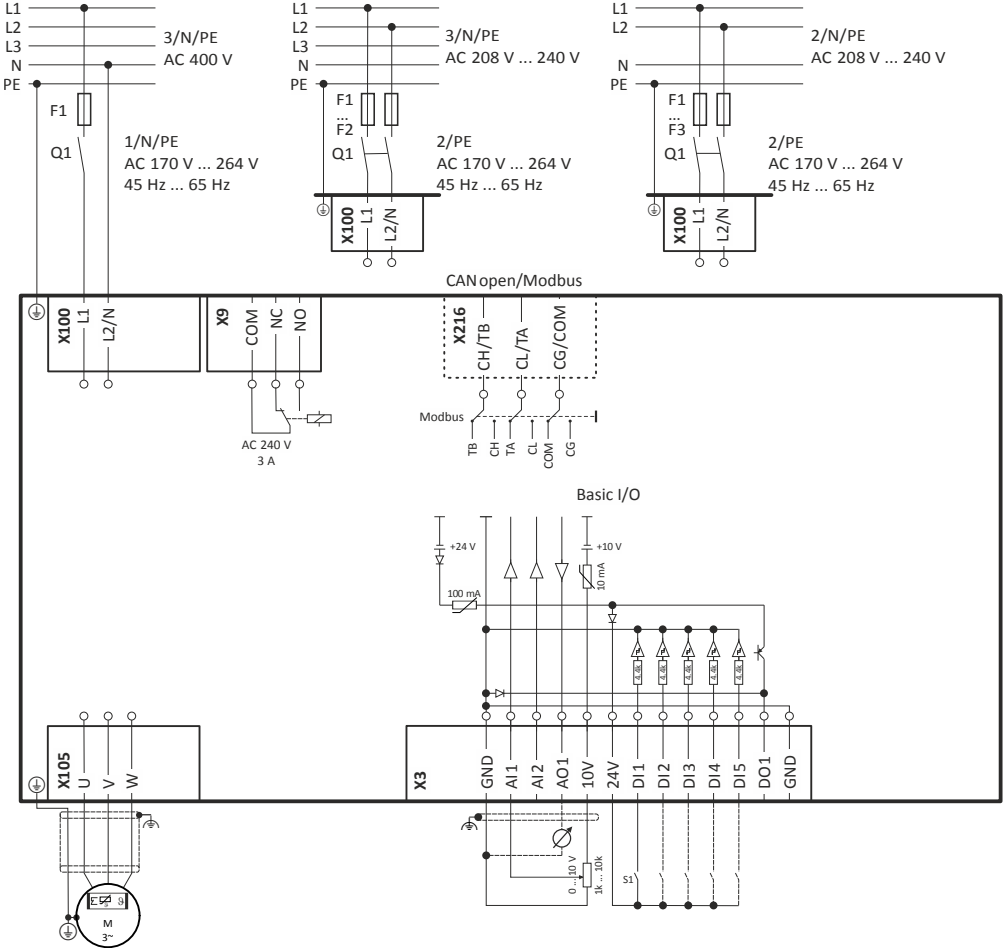
Fig. 7: Wiring example
