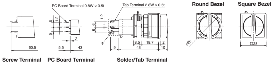
Screw Terminal PC Board Terminal Solder/Tab Terminal
