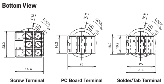
Screw Terminal PC Board Terminal Solder/Tab Terminal
