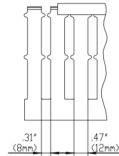
SIDE SECTION
