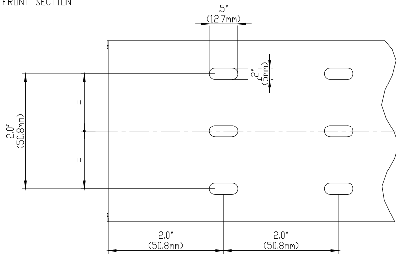
BASE PERFORATION
