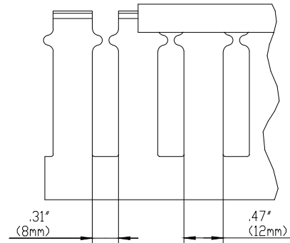
SIDE SECTION
