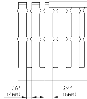
SIDE SECTION
