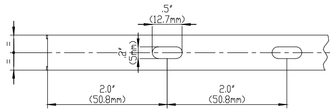
BASE PERFORATION
