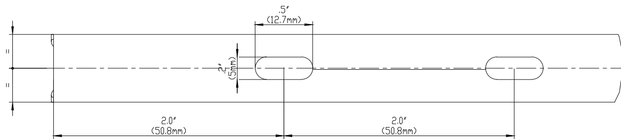
BASE PERFORATION
