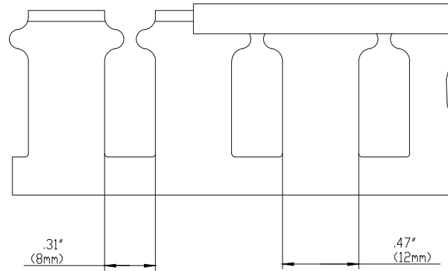
SIDE SECTION
