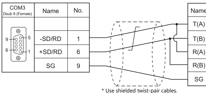
Wiring diagram 3 - COM3
