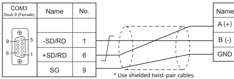
Wiring diagram 1 - COM3
