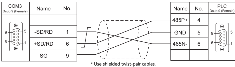
Wiring diagram 4 - COM3
