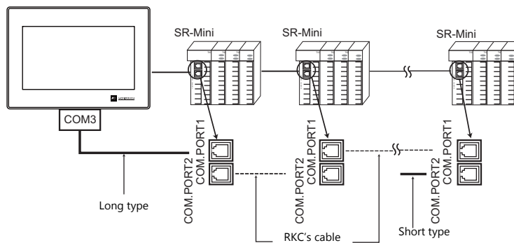
Wiring diagram 3 - COM3
