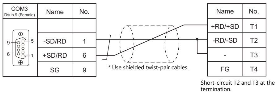
Wiring diagram 1 - COM3
