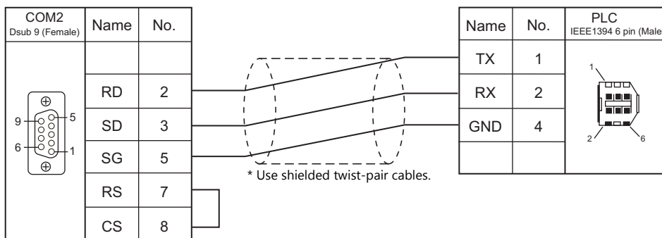
Wiring diagram 1 - COM2
