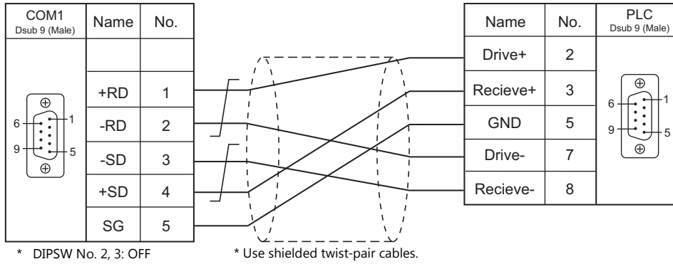
Wiring diagram 1 - COM1
