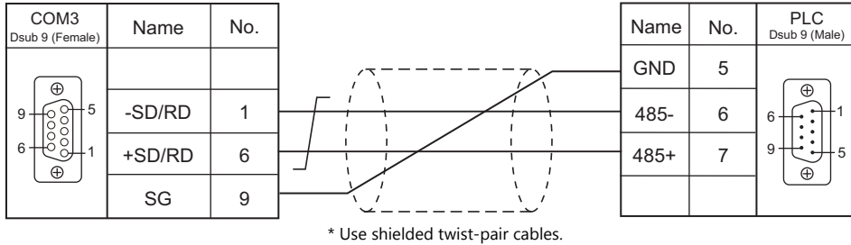
Wiring diagram 1 - COM3
