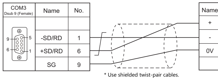
Wiring diagram 1 - COM3
