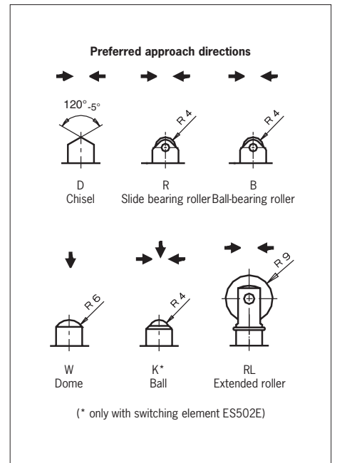
Fig. 4: Plungers and approach directions
