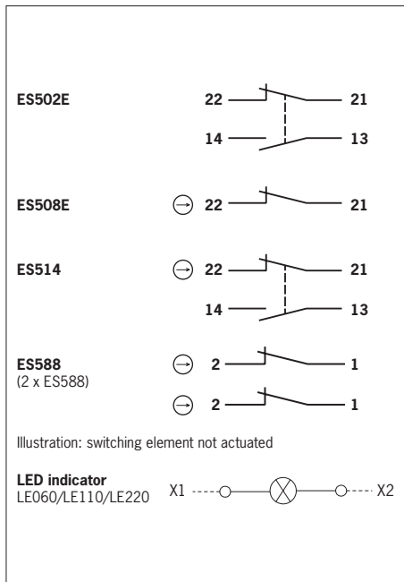
Fig. 2: Switching elements and terminal assignment
