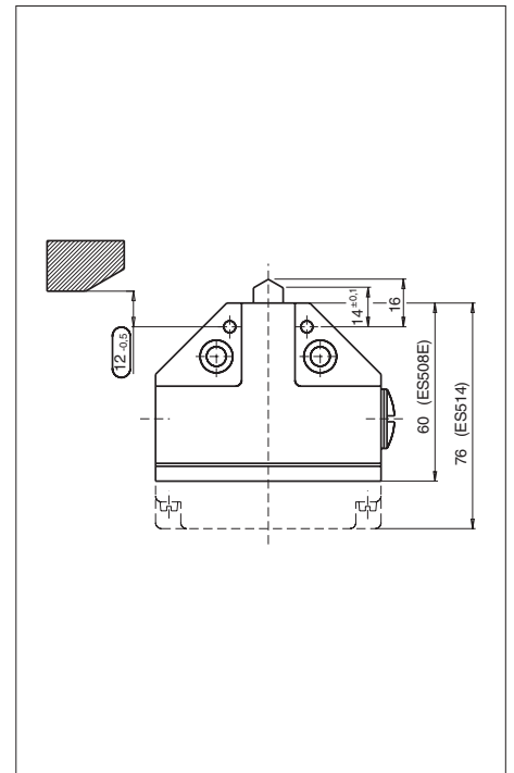
Fig. 6: Dimension drawing for N1A.508/...514
