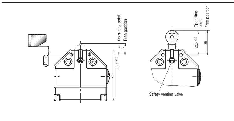
Fig. 7: Dimension drawing for N1A.2588 (2 x ES588)
