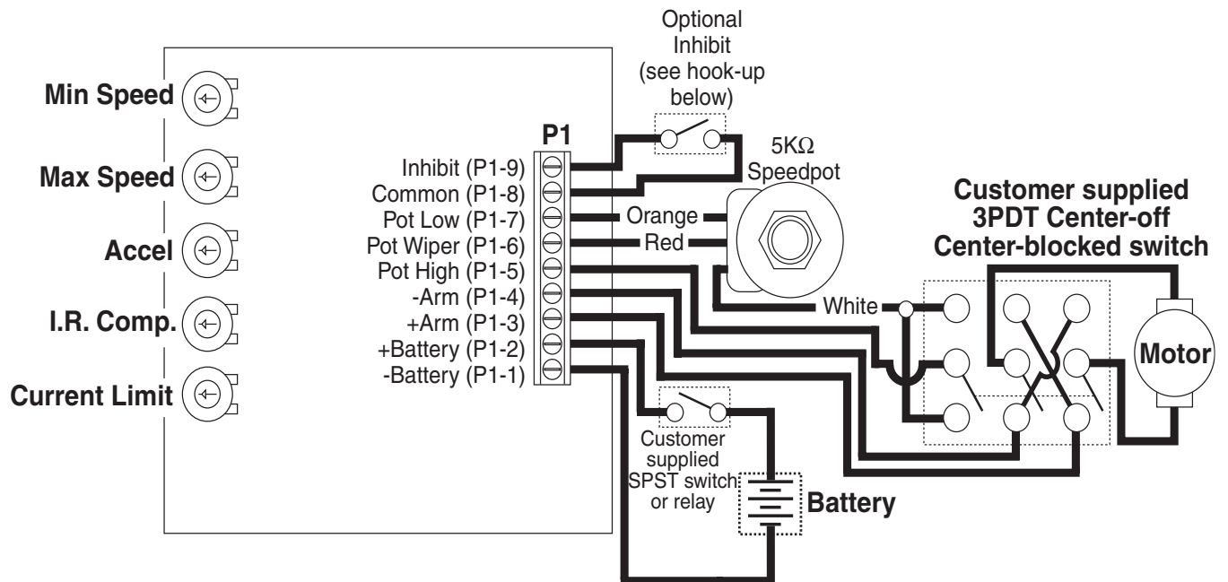
65E10 REVERSING HOOK-UP DIAGRAM
