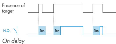
On delay
