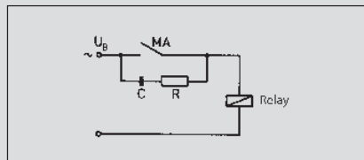
Suppression of voltage peaks with RC element
