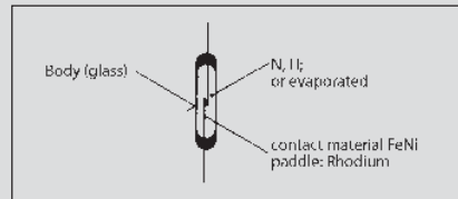
Design of a reed contact
