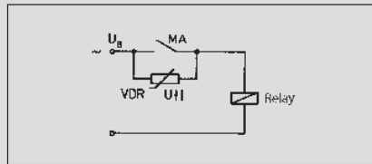
Suppression of voltage peaks with a VDR
