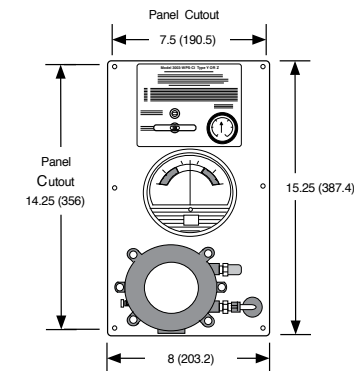
WPS/WPSA VM Configuration Front View
