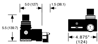
Side View Model 3004 CK System Panel Cutout Pattern
