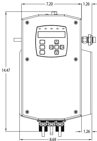
6000 Control unit with housing
