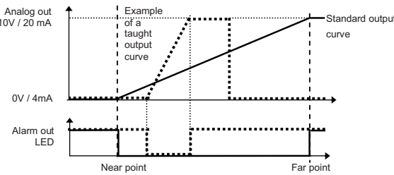
Example of a taught measuring range: 4 mA / 0 V in the near point, 20 mA / 10 V in the far point
