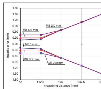
typical linearity error
