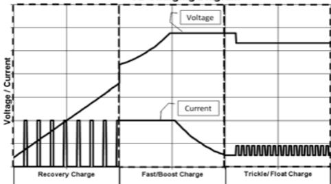
CB Charging Diagram
