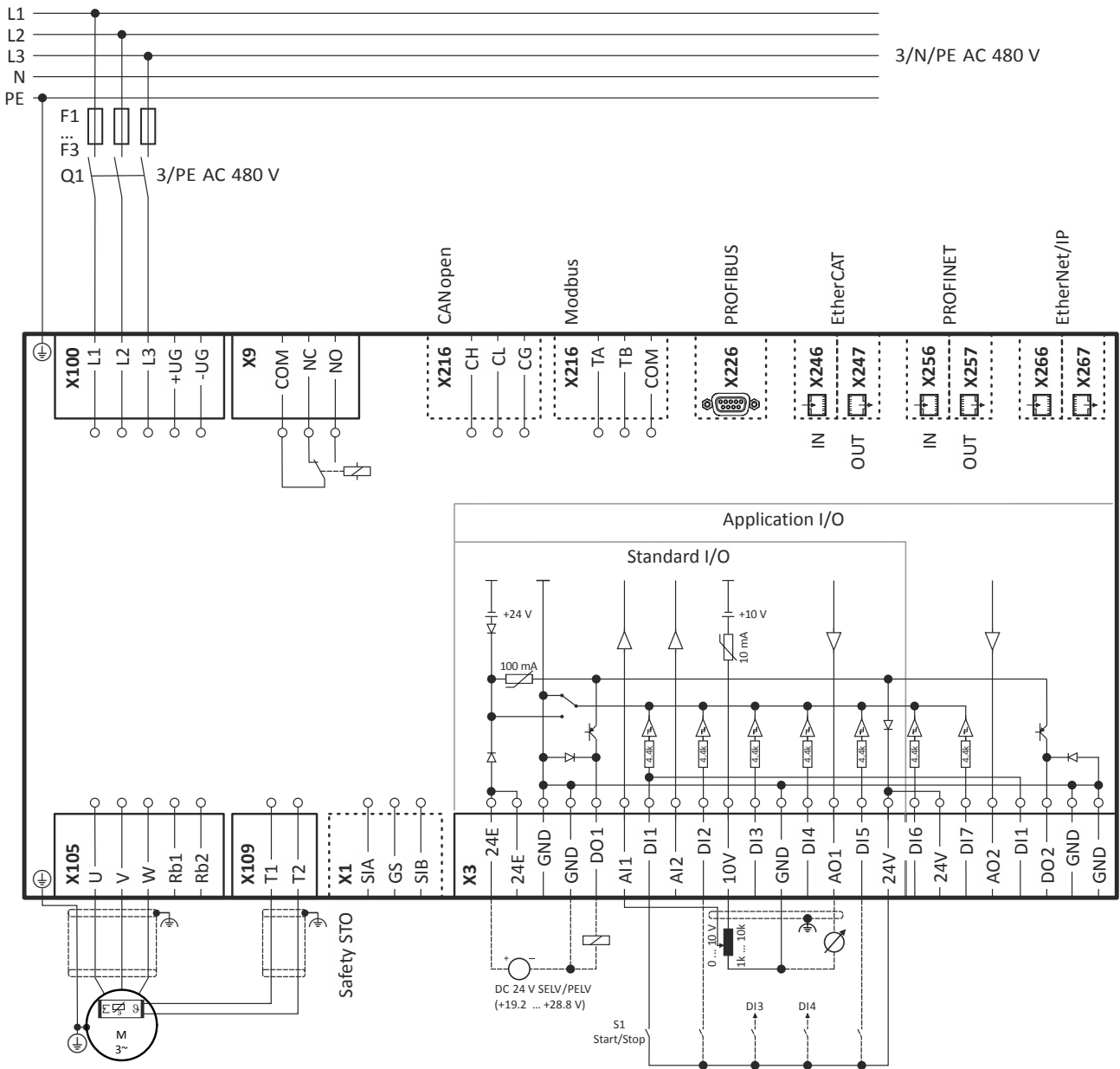
Fig. 9: Wiring example
